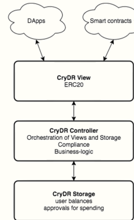
Figure 3. Tiered Architecture
