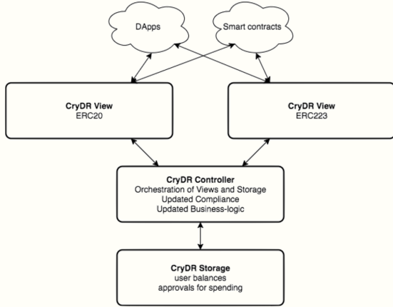
Figure 5. View Upgrades
