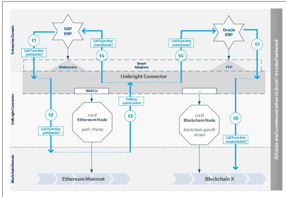
Figure 9: The Unibright Connector Architecture
