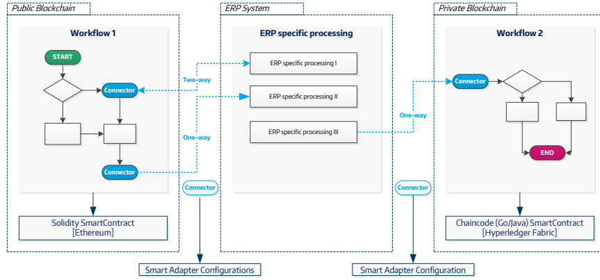
Figure 11: Orchestrating workflows
