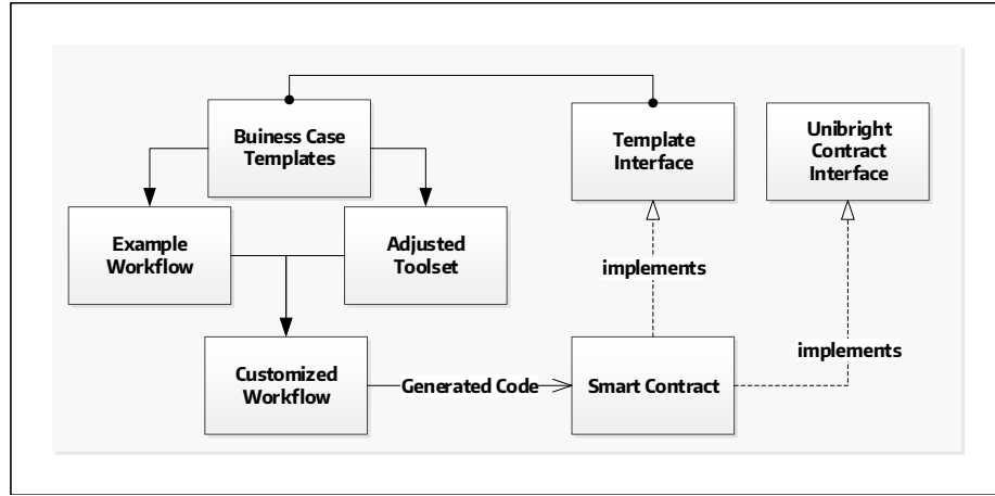
Figure 4: Inheritance Hierarchy
